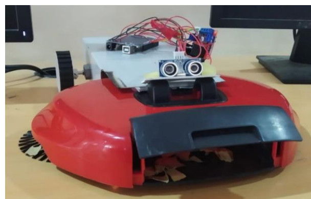
Figure: Automated MOP for floor cleaning using IoT
